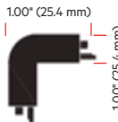
3" 90° PolyBostylene® Corner Cap 144 pieces per box PBCN3000-XXX
