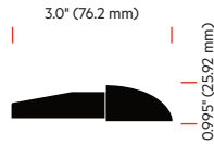
2" Round PolyBostylene® End Cap 144 pieces per box PBER2000-XXX
