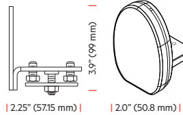
Flat End Cap Cast Aluminum BBEC
