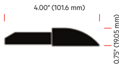
3" Round PolyBostylene® End Cap 144 pieces per box PBCN3050-XXX
