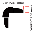
2" 90° PolyBostylene® Corner Cap 144 pieces per box PBCN2000-XXX
