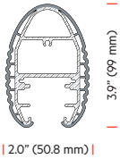
Aluminum Rail Rigid Vinyl Cover BBRA-144-XXX 144 denotes length in inches
