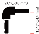
1" 90° PolyBostylene® Corner Cap 144 pieces per box PBCN1000-XXX
