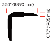
3" 90° PolyBostylene® Corner Cap 144 pieces per box PBCN3050-XXX
