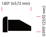
2" Flat PolyBostylene® End Cap 144 pieces per box PBEF2000-XXX
