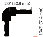
1" 90° PolyBostylene® Corner Cap 144 pieces per box PBCN1000-XXX
